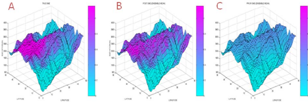
Figure 2. Synthetic experiment over 25-25 km domain in Sequoia National Park showing “true” snow water equivalent (A), posterior snow water equivalent after assimilation of MODIS snow cover images (b), and prior snow water equivalent from the open loop simulation (c). Note the clear improvement in SWE estimation with the inclusion of the MODIS data as evident in the closer match of B to A relative to C to A.
